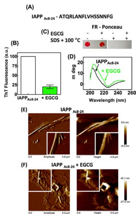
Figure 5. Amyloid remodeling activity of EGCG on IAPP fibrils. Mature IAPP Ac8-24 (A) amyloid fibrils (65 mg/mL) were incubated in the absence or presence of 30 \mu M EGCG for 24 h at 25 °C. After the centrifugation/wash protocol, the ThT fluorescence (B), CD (D), and AFM images (E,F) were recorded. Insets of panels E and F: each image is 2 \mu m \times 2 \mu m. An aliquot of these samples was boiled or not in 2% SDS and then applied to FR membrane that was stained by Ponceau (C).
