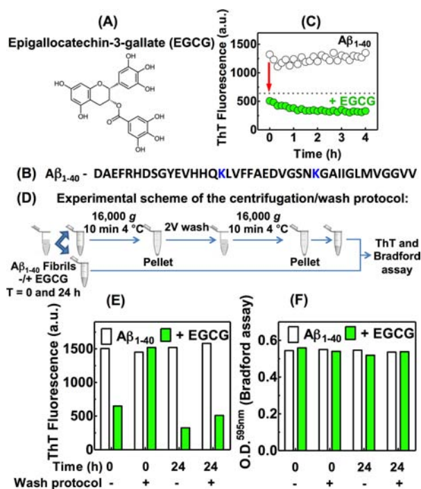
Figure 1. Effect of EGCG on ThT fluorescence of A\beta_{1-40} amyloid fibrils. (A) Structure of EGCG. (B) Primary sequence of A\beta_{1-40} peptide; lysines 16 and 28 are highlighted in blue. (C) Kinetics of A\beta_{1-40} amyloid fibril remodeling monitored by ThT fluorescence incubated in the absence or presence of EGCG. (D) Experimental scheme of the centrifugation/wash protocol. (E) ThT fluorescence or (F) protein quantification by the Bradford assay (OD) of samples incubated for 0 or 24 h in the absence or presence of EGCG. The use of the centrifugation/wash protocol is denoted by (+). The buffer used for all assays was 50 mM phosphate buffer pH 7.4, 150 mM NaCl (25 °C). [ A\beta_{1-40} amyloid fibrils] = 65 \mu\text{g}/\text{mL} , [EGCG] = 30 \mu\text{M} . For ThT fluorescence, the ThT concentration used was 20 \mu\text{M} , E_x = 440 nm and E_m = 485 nm.
