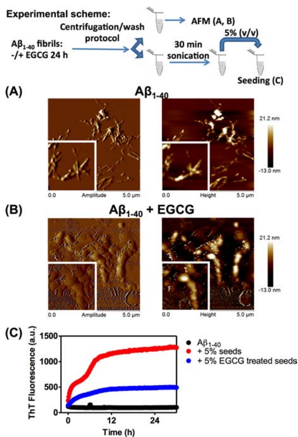
Figure 2. Effect of EGCG on the morphology and seeding activity of A\beta_{1-40} . A\beta_{1-40} (65 \mu\text{g}/\text{mL} ) fibrils were incubated in the absence or presence of 30 \mu\text{M} EGCG for 24 h at 25 °C. The fibrils were processed using the centrifugation/wash protocol, and one aliquot was used for AFM analysis (panels A and B), while the other aliquot was sonicated for 30 min in order to produce fragmented fibrils used in the seeding experiment (panel C). AFM images of A\beta_{1-40} fibrils incubated in the absence (A) or presence (B) of EGCG. The left images represent the amplitude image, while the right images represent the height images. Insets: each image is 2 \mu\text{m} \times 2 \mu\text{m} . (C) A monomeric solution of A\beta_{1-40} peptide (65 \mu\text{g}/\text{mL} ) was incubated in the absence or presence of 5% seeds in 50 mM phosphate buffer pH 7.4 and 150 mM NaCl without agitation. The seeds were produced by sonication of A\beta_{1-40} amyloid fibrils incubated in the absence or presence of EGCG (30 \mu\text{M} ) for 24 h at 25 °C. The samples containing ThT (20 \mu\text{M} ) were incubated at 25 °C in a 96-well plate, and every 10 min the fluorescence (excitation at 440 nm, emission at 485 nm) was monitored.
