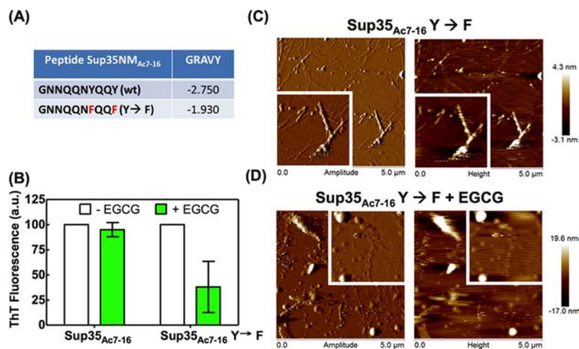
Figure 7. EGCG is incapable of remodeling Sup35NM Ac7-16 amyloid fibrils. (A) Primary sequence of the peptides comprising Sup35NM Ac7-16 (wt) and Sup35NM Ac7-16 Y→F amyloid fibrils as well as the grand average of hydrophobicity index (GRAVY) of these peptides. (B) Sup35NM Ac7-16 or Sup35NM Ac7-16 Y→F mature amyloid fibrils (65 μg/mL) were incubated in the absence or presence of 30 μM EGCG for 24 h at 25 °C. After the centrifugation/wash protocol, the ThT fluorescence was recorded. (C,D) AFM images of Sup35NM Ac7-16 Y→F mature amyloid fibrils incubated in the absence (C) or presence (D) of EGCG. Insets: each image is 2 μm × 2 μm.
