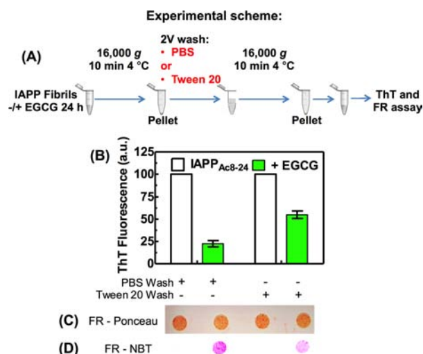
Figure 6. Amyloid remodeling activity of EGCG is still partially functional in the presence of detergent micelles. (A) Experimental scheme of the centrifugation/wash protocol, highlighting the wash step performed with PBS or PBS containing Tween 20. IAPP Ac8-24 mature amyloid fibrils (65 μg/mL) were incubated in the absence or presence of 30 μM EGCG for 24 h at 25 °C. After the centrifugation/wash protocol (A), the ThT fluorescence (B) was recorded. An aliquot of these samples (without boiling) was then applied to FR membrane that was stained by Ponceau (C) or NBT (D).
