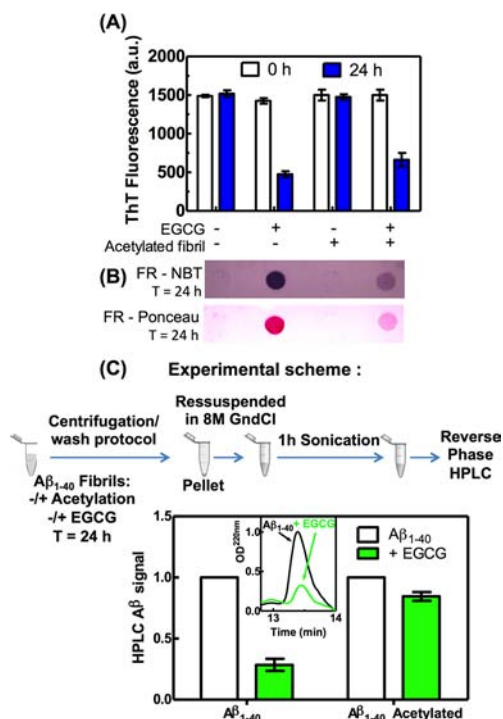
Figure 4. Amyloid remodeling activity of EGCG does not require free amines. Acetic anhydride was used to acetylate any free amines in the A\beta_{1-40} fibrils. The acetylated fibrils were incubated in the absence or presence of EGCG for 24 h and the ThT fluorescence using the centrifugation/wash protocol (A), and the FR assay stained with NBT or Ponceau (B) were monitored. Non-acetylated fibrils were used as control. (C) Acetylated and non-acetylated A\beta_{1-40} amyloid fibrils were incubated in the absence or presence of 30 \mu M EGCG for 24 h. After the centrifugation/wash protocol, the pellets were resuspended in 8 M guanidine hydrochloride (GndCl) and sonicated for 1 h. The samples were analyzed by RP-HPLC, monitoring the optical density at 220 nm (inset, non-acetylated fibril). The HPLC A\beta signal was calculated from the area under the peak.
