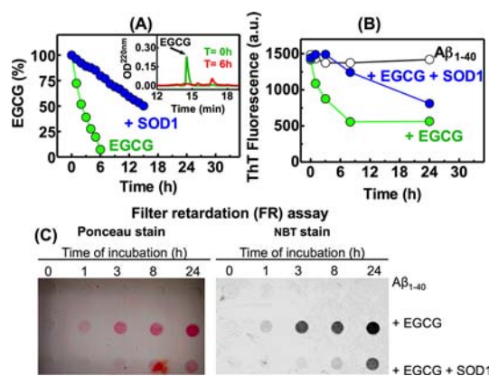
Figure 3. EGCG amyloid remodeling activity depends on auto-oxidation. (A) The stability of EGCG is enhanced in the presence of 1 \mu\text{g}/\text{mL} SOD1. (Inset A) The auto-oxidation of EGCG was monitored by RP-HPLC using a C18 column. (B) A kinetics experiment monitoring the ThT fluorescence using the centrifugation/wash protocol was performed with A\beta_{1-40} amyloid fibrils in the presence of EGCG or EGCG + SOD1. Buffer alone was used as a control. (C) Filter retardation assay of aliquots of the samples described in Figure 3B stained by Ponceau or NBT, as indicated. For detailed experimental conditions see the legend of Figure 1.
